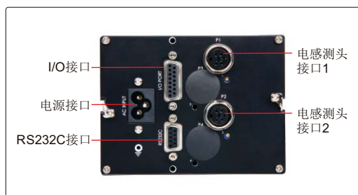
显示器背面(7105-DA2)
