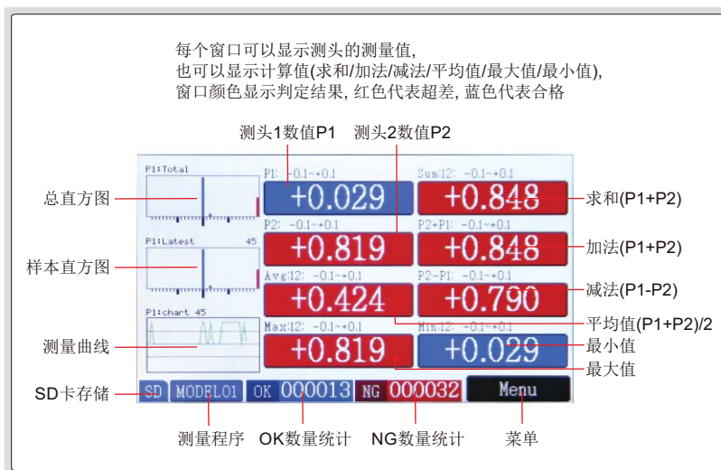
测量界面(7105-DA8)
